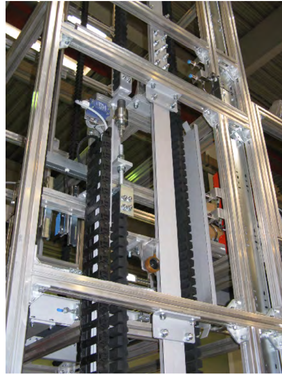
Energy chain, guide profiles, lifting carriage and chain damage monitoring
